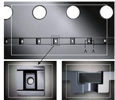
Pocket View A-A
