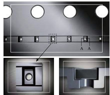
Polycarbonate Precision Solder Sphere Carrier Tape for Solder Balls
