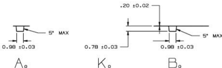
Carrier Tape Dimensions for 0.030" Solder Balls
